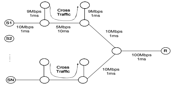
Figure 1. Simulation topology
