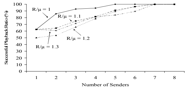
Figure 5. Successful playback ratio for NLANR PMA traces
