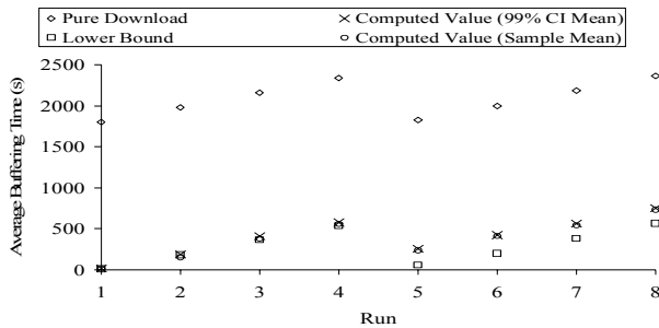
Figure 8. Average buffering time for different simulation runs
