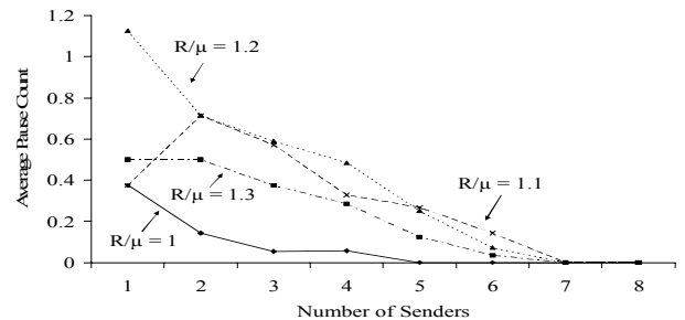
Figure 6. Average pause count for NLANR PMA traces
