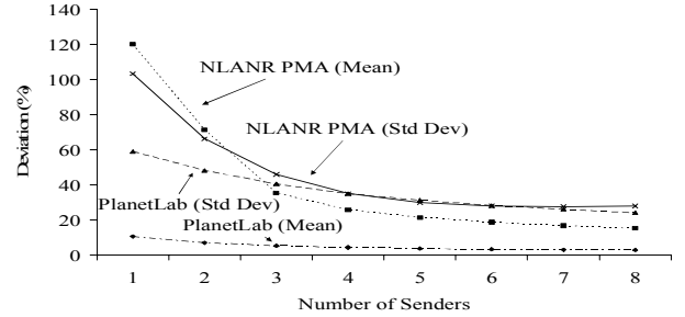
Figure 2. Deviation of mean and standard deviation from initial estimations
