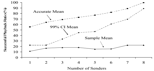
Figure 4. Comparison of successful playback ratio when using Sample Mean, 99% CI Mean, and Accurate Mean (PlanetLab traces)
