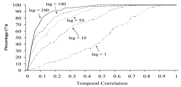
Figure 3. The CDF of temporal correlation with different lag values
