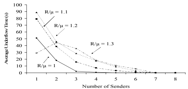
Figure 7. Average underflow time for NLANR PMA traces
